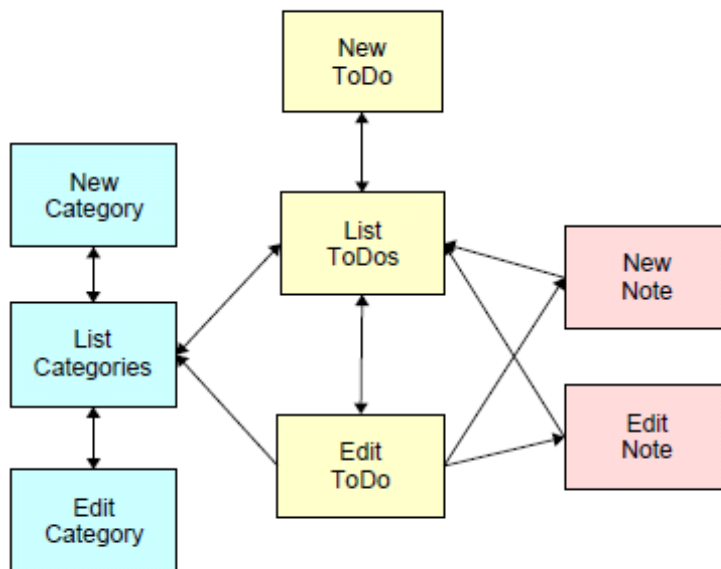
Illustration 9 Navigation paths through the Application
